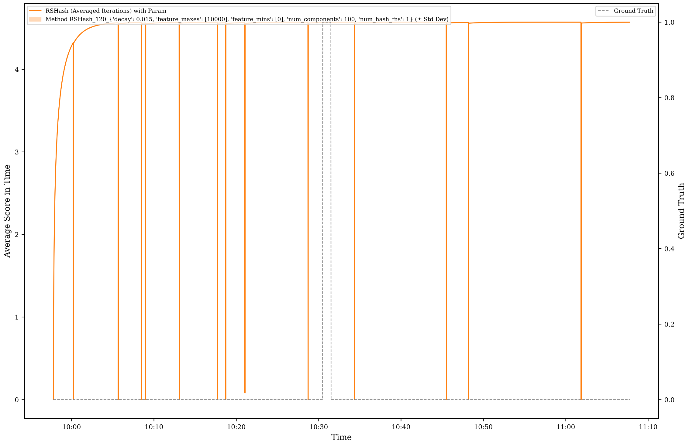
Method RSHash Score for Scenario A4
